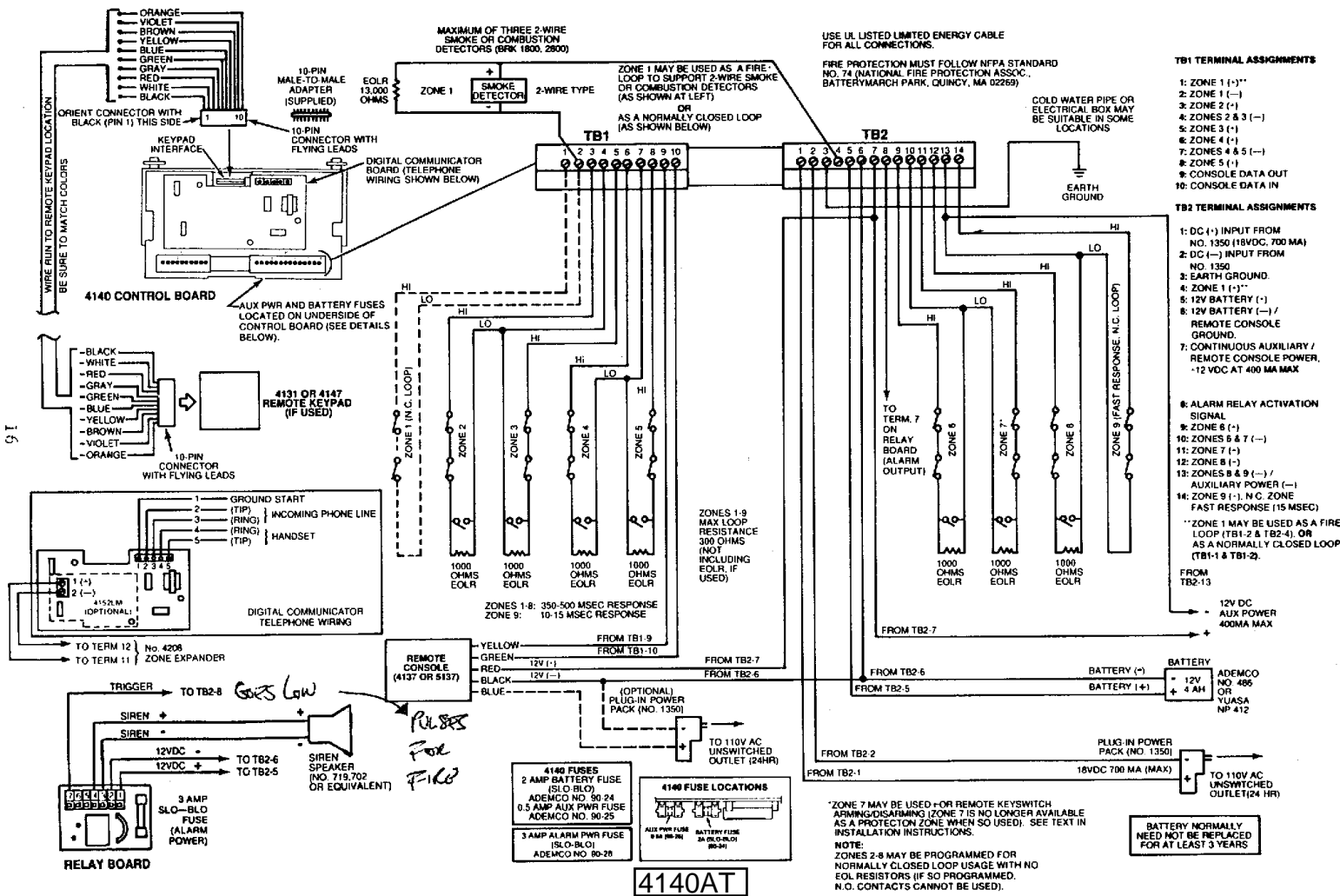
Diagram 1. SUMMARY OF CONNECTIONS
